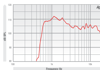
Frequency response curve of the horn measured on axis at distance of 1 meter with 1 watt signal with CD-314 compression driver.
