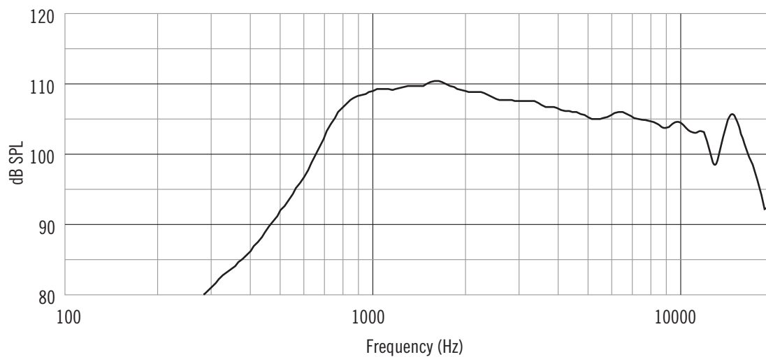
Response 1W/1m
