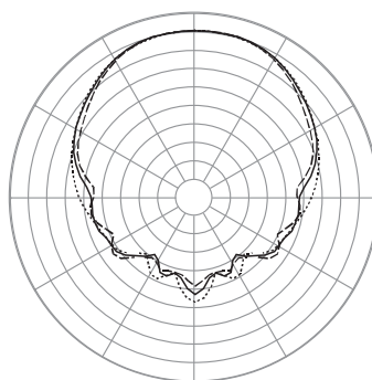
Horizontal 4000 Hz 1/3 Octave Polars
